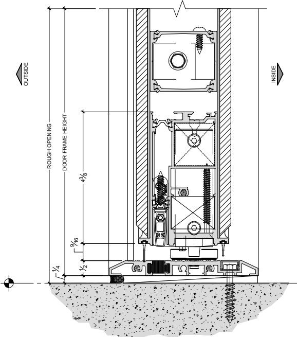
3 SECTION DETAIL - ES-PSD5030T - SILL OPTION 3 SCALE: 6" - 0" = 1' - 0"
